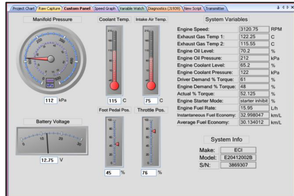
Program screenshot
