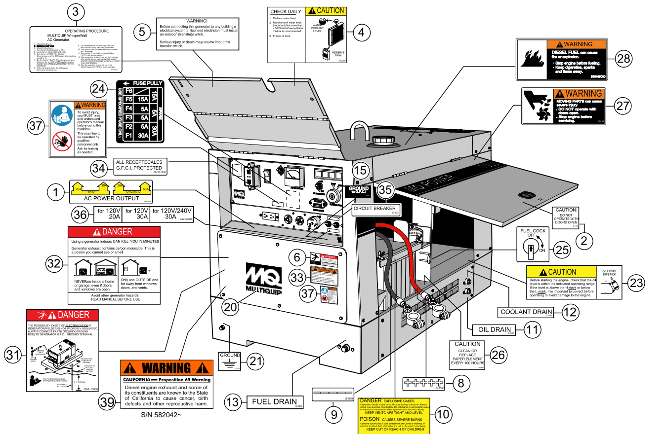
FRONT VIEW
