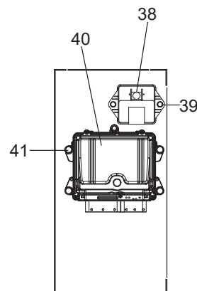
VIEW-B
