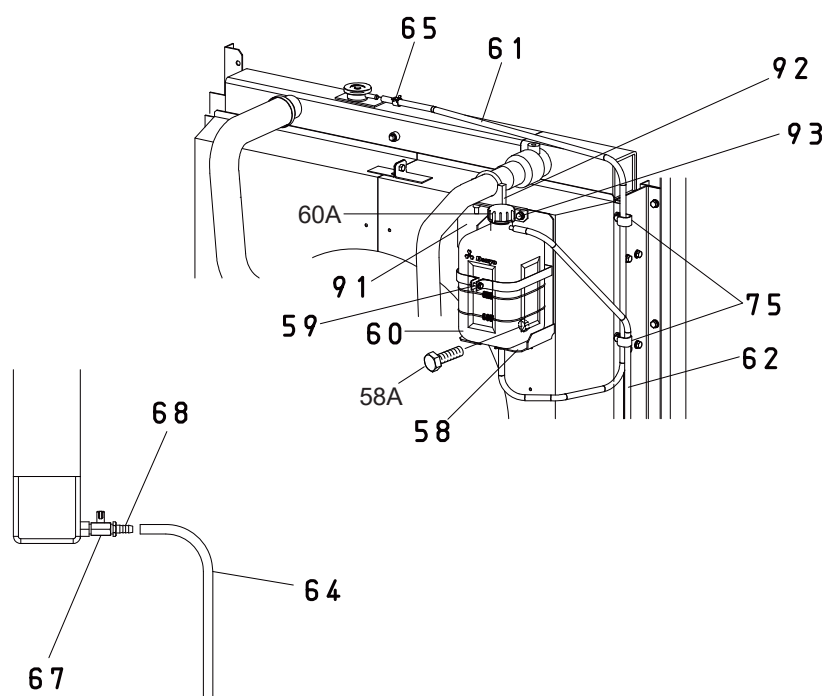
VIEW-B
