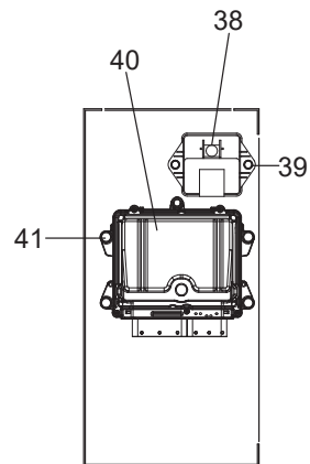
VIEW-B
