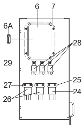
VIEW-A
