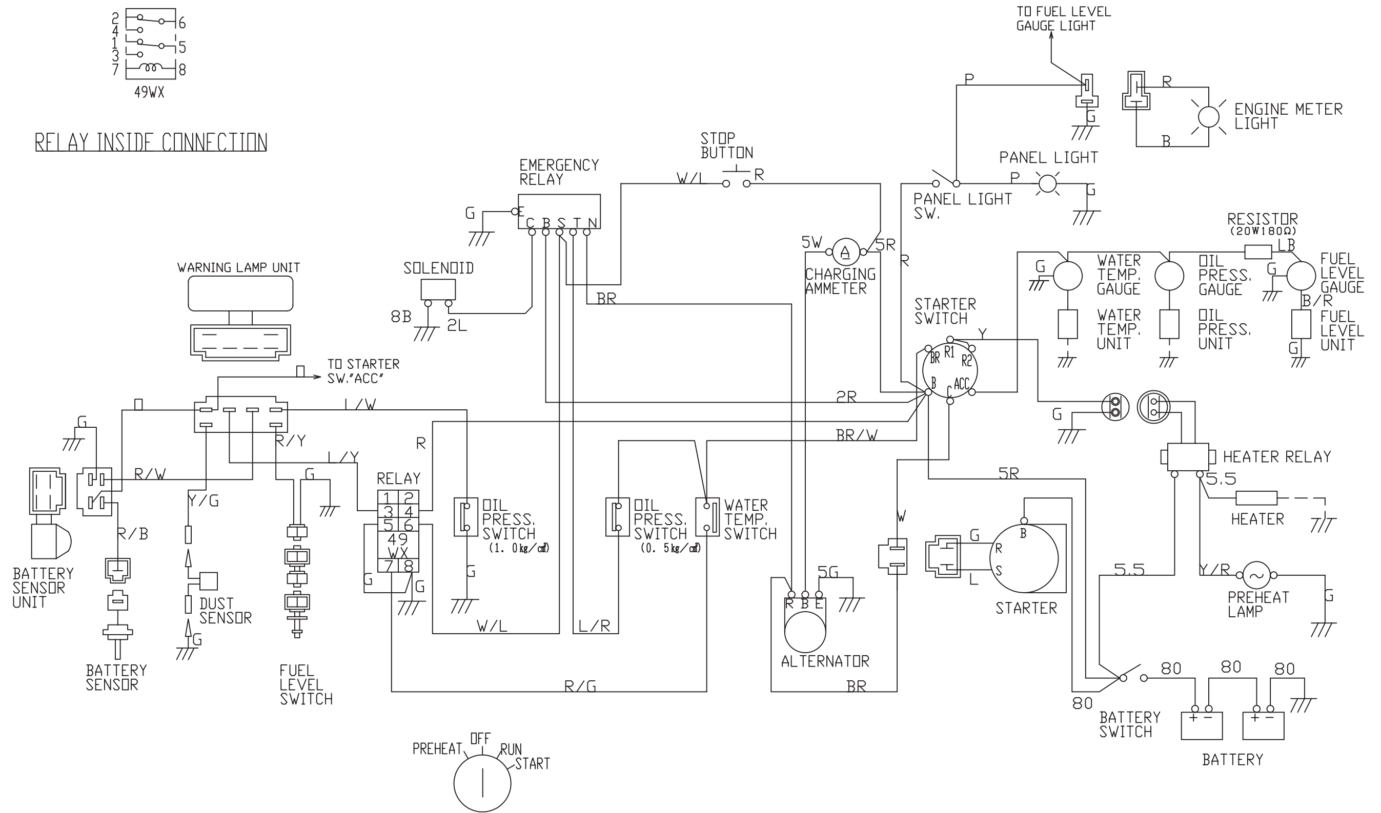
STARTER SWITCH
