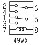
RELAY INSIDE CONNECTION
