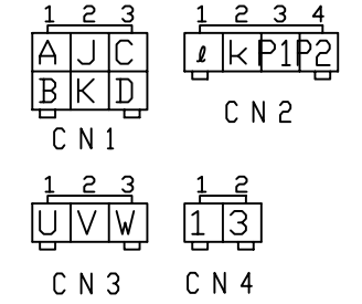
AVR CONNECTOR (View from inserting wire side)
