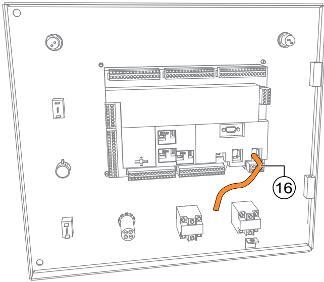
BASLER CONTROL PANEL (REAR)
