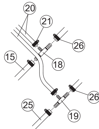
DETAIL - C
