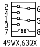
RELAY INSIDE CONNECTION
