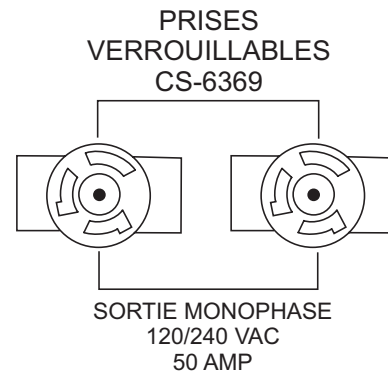
Figure 8. 120/240V Prises Secondaires Verrouillables
