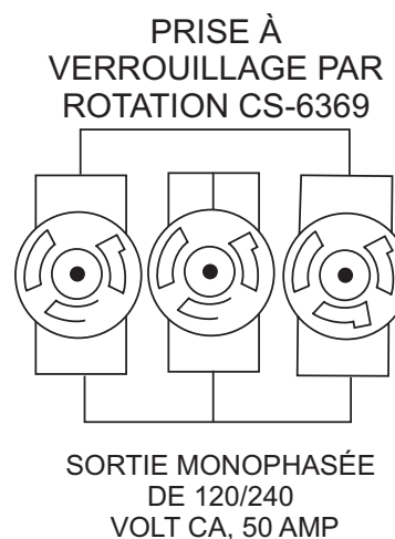
Figure 8. 120/240V Prises Secondaires Verrouillables
