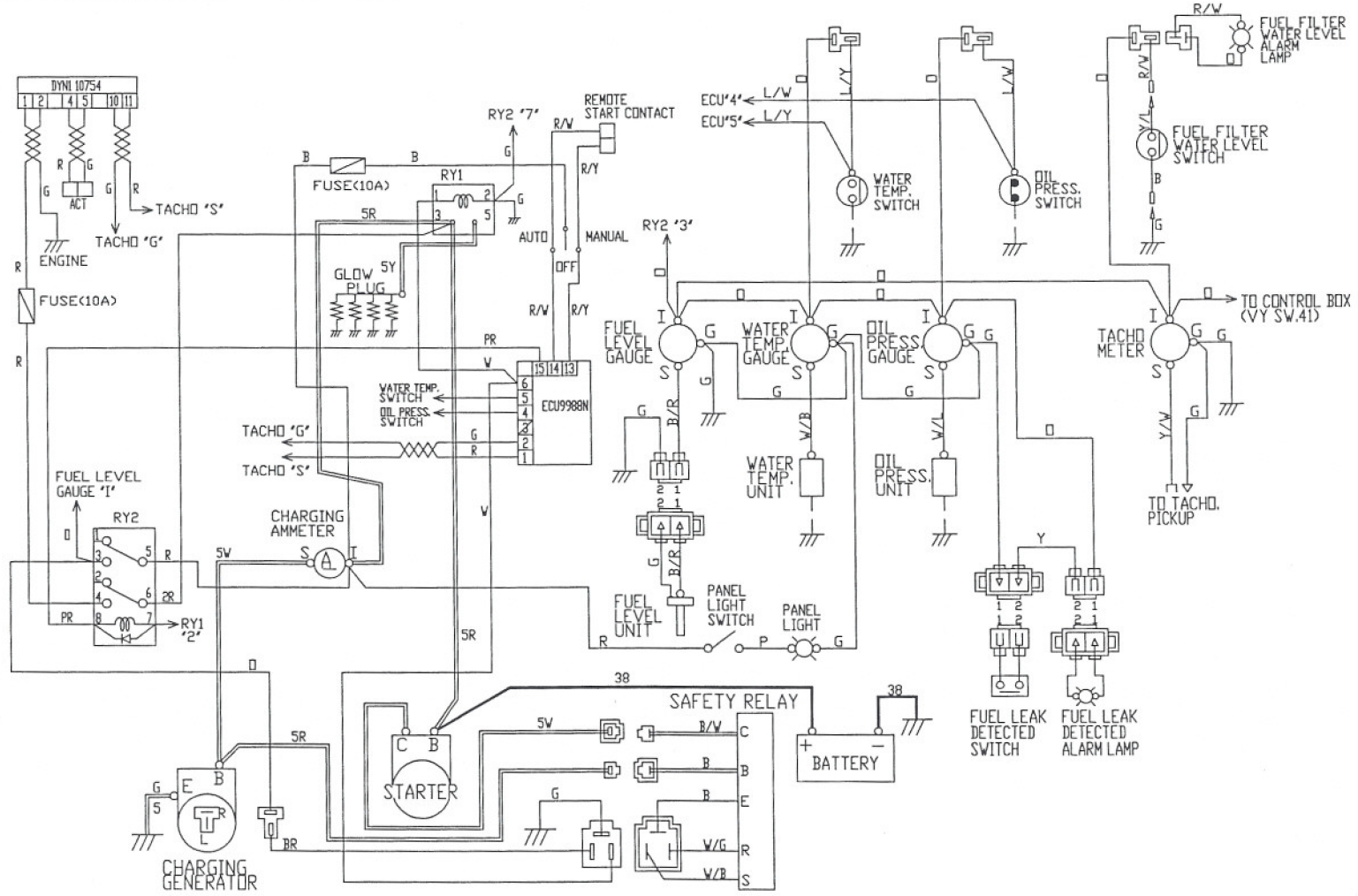
DCA45USI WITH ECU/EGS ENGINE WIRING DIAGRAM
