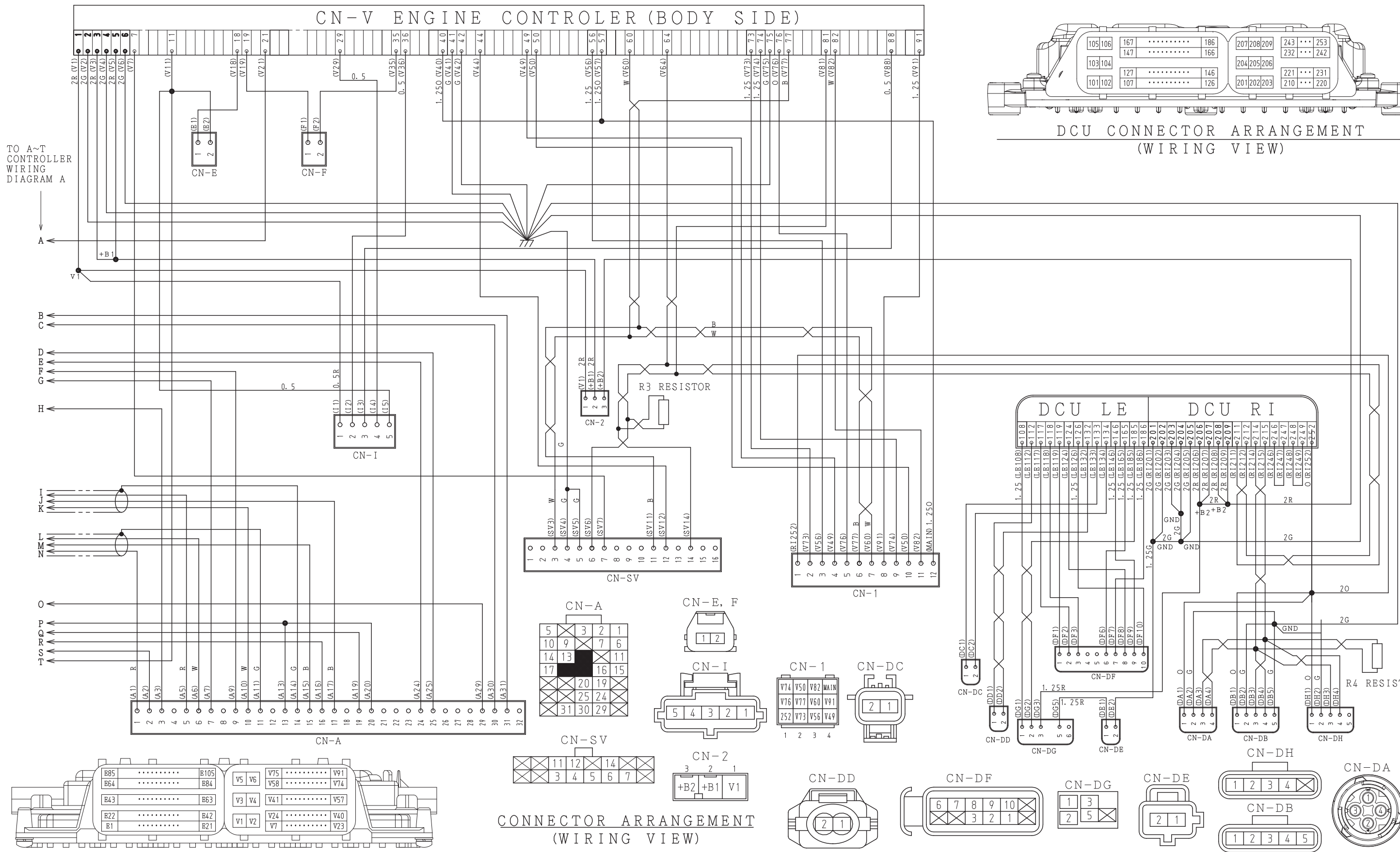
ECM CONNECTOR ARRANGEMENT (WIRING VIEW)
