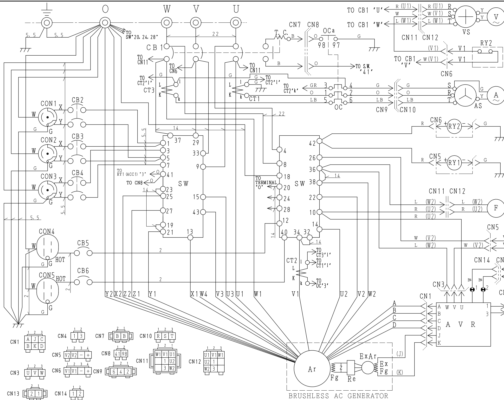
CONNECTOR ARRANGEMENT (WIRING VIEW)
