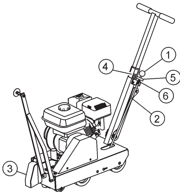
Figure 13. Raise/Lower Assembly
