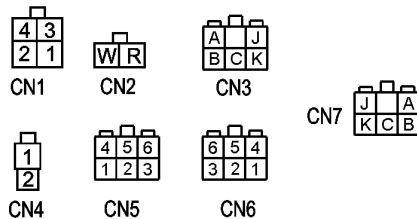
CONNECTOR ARRANGEMENT (VIEW FROM INSERTING WIRE SIDE)
