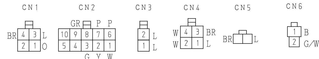
Connector (View from Inserting Wire side)
