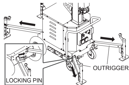
Figure 7. Extending Outriggers
