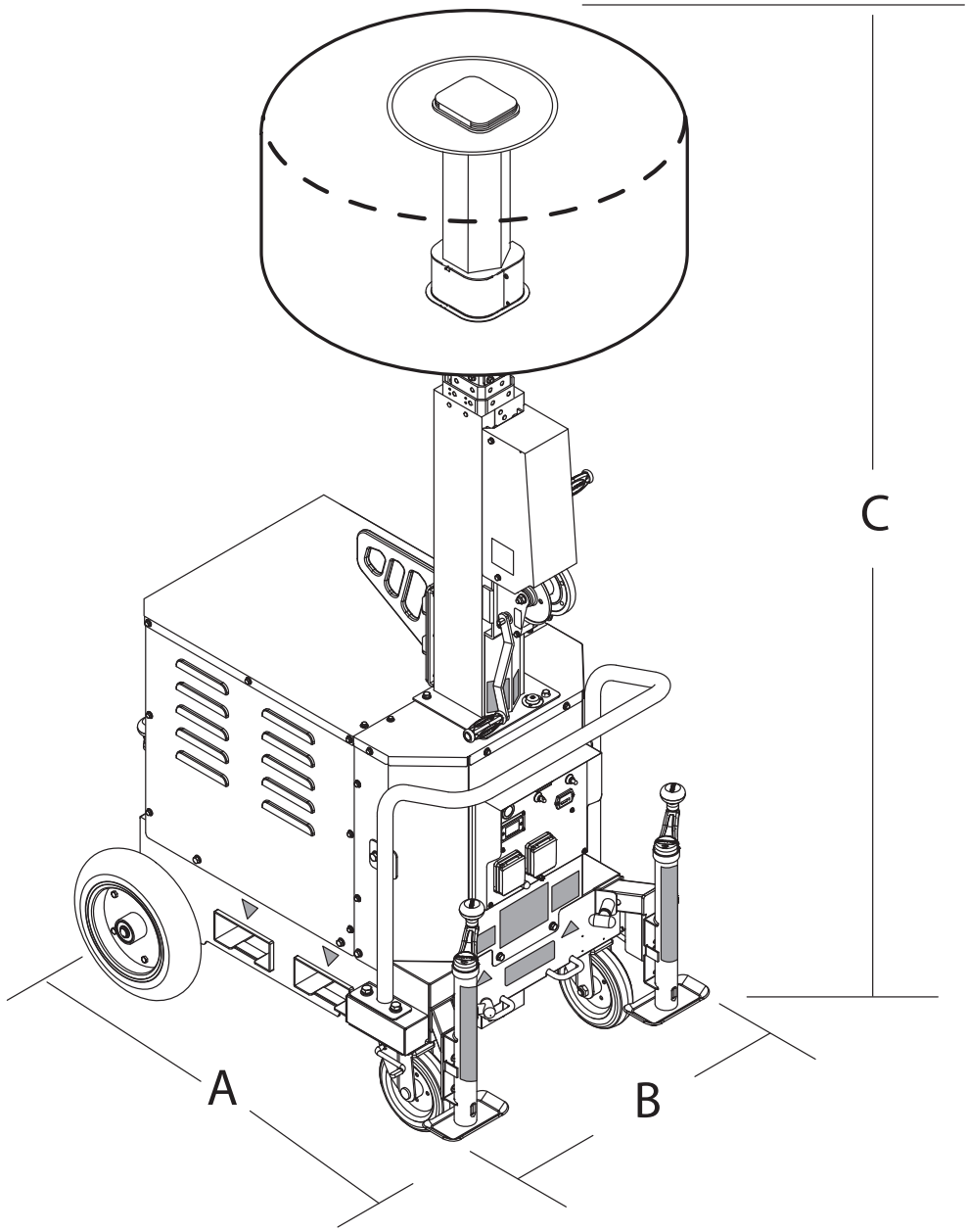
Figure 1. GBBAT8BM Dimensions
