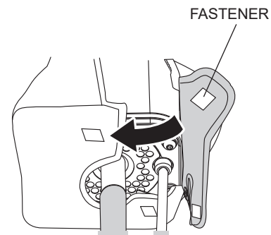
Figure 28. Loop Fastener
