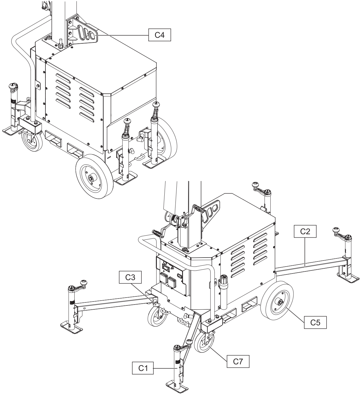
Figure 42. Cart Maintenance
