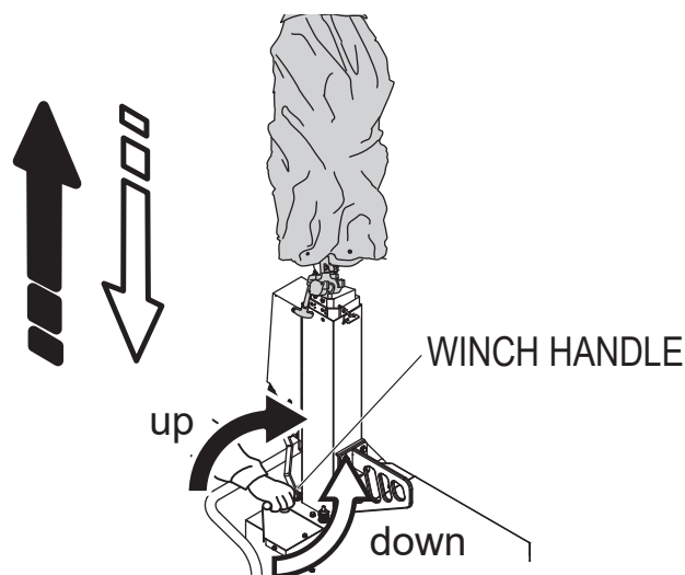
Figure 13. Raising and Lowering Mast
