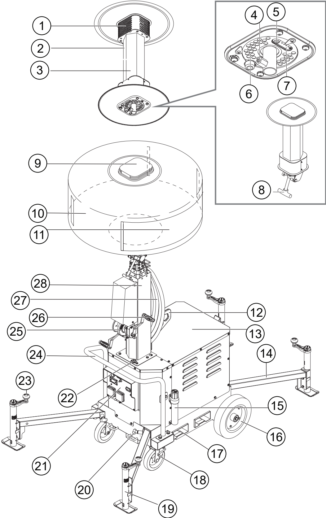
Figure 4. GBBAT8BM Components
