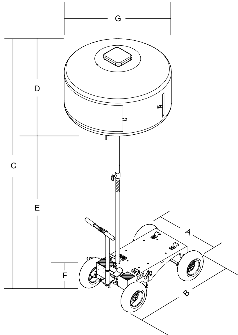
Figure 1. GBC8LED Dimensions
