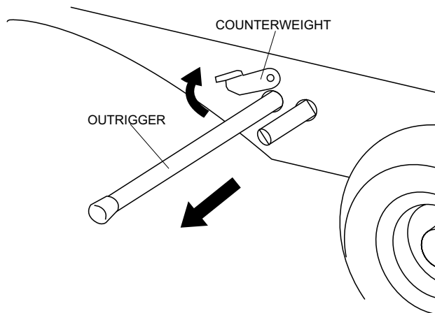
Figure 14. Deploying Outrigger
