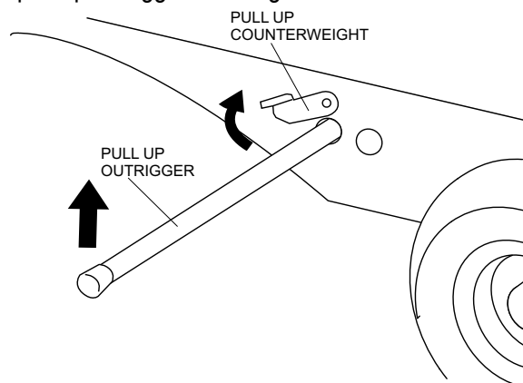
Figure 16. Stowing Outrigger
