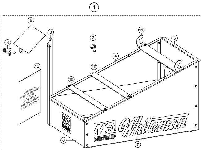
Figure 1. J-B Walk-Behind Trowel Stand Assembly Kit
