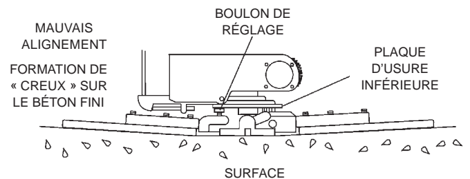
Figure 18. Plaque de tripode usée
