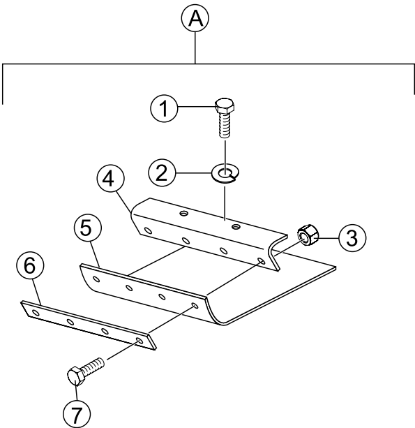
Figure 1. Kit Parts
