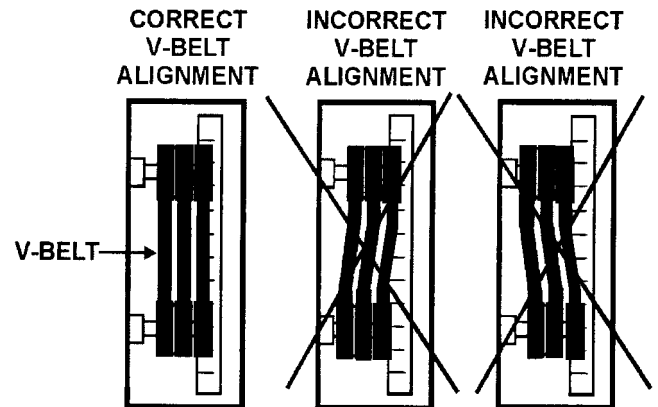
Figure 5. Pulley Alignment
