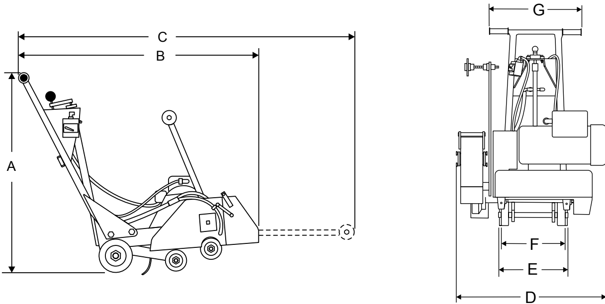
Figure 1. SP1E16A Dimensions
