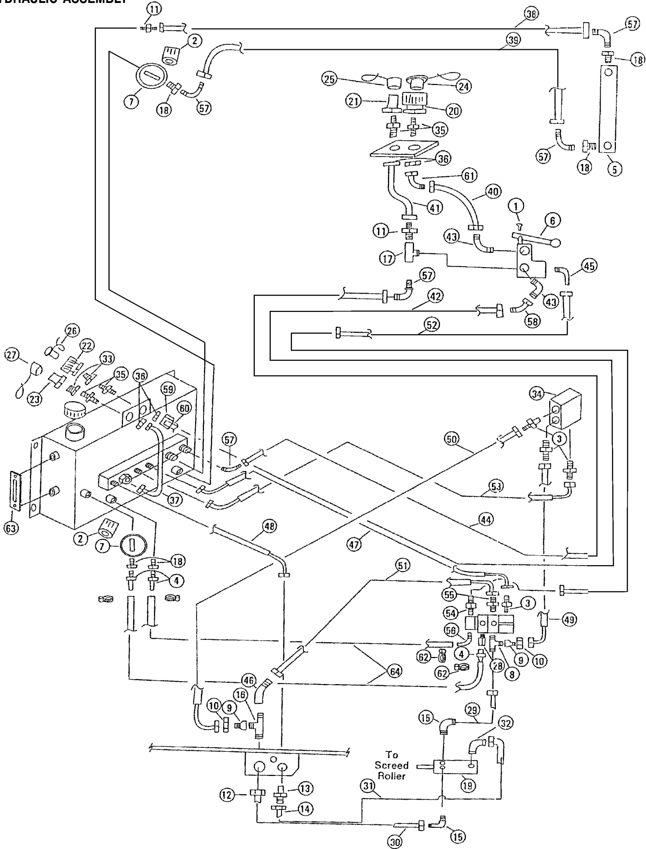
WRS 5200 RIDE-ON ROLLER SCREED see legend on next page
