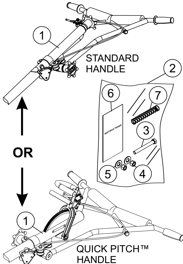
Figure 1. Standard/Quick Pitch™ Trowel Handle
