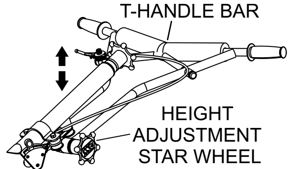
Figure 4. T-Handle Bar Adjustment
