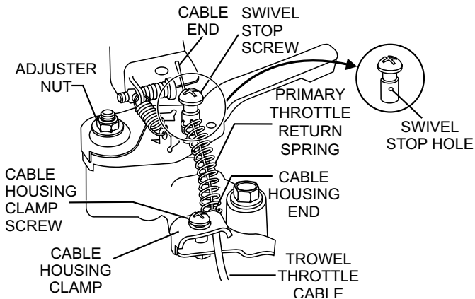
Figure 9. Throttle Cable Installation
