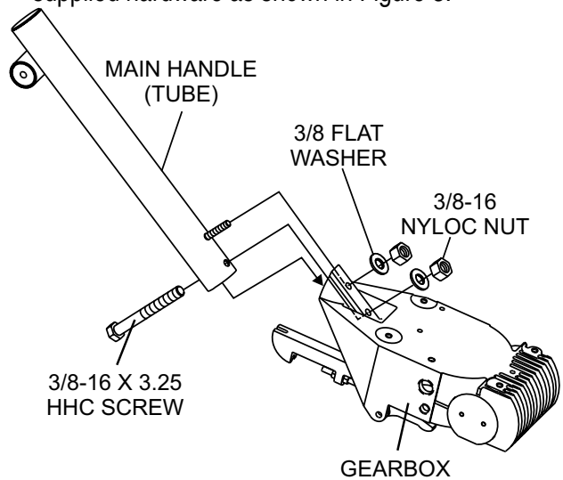
Figure 3. Handle Installation
